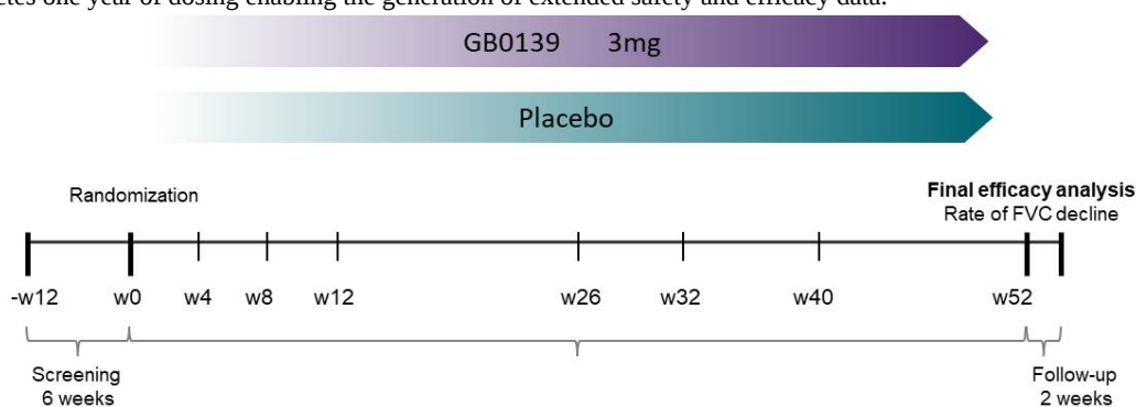
Figure 6. Ongoing GALACTIC-1 trial design
